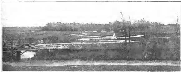
B. Meandering stream and ox-bow lake. (Photo by Neal.)
